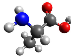
Protein Subunit C_3H_7O_2N
