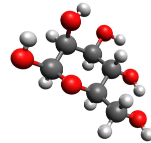
Carbohydrate Subunit C_6H_{12}O_6
